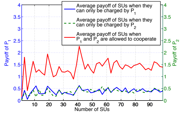
Fig. 7. Average payoff of SUs for different numbers of SUs.
