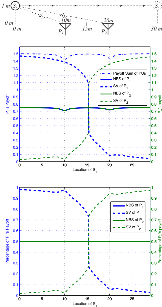
Fig. 10. The payoff divisions between P_1 and P_2 on two fairness criteria: Nash bargaining solution (NBS) fairness and Shapley value (SV) fairness.
